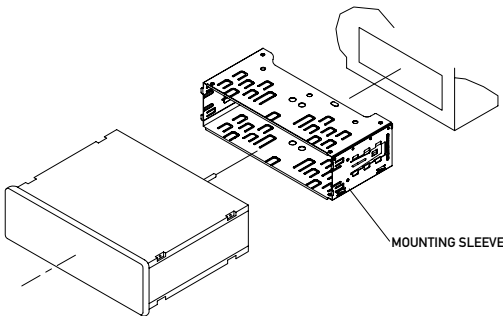
TYPICAL FRONT-LOAD DIN MOUNTING METHOD
